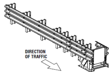
T – connection to Thrie Beam
